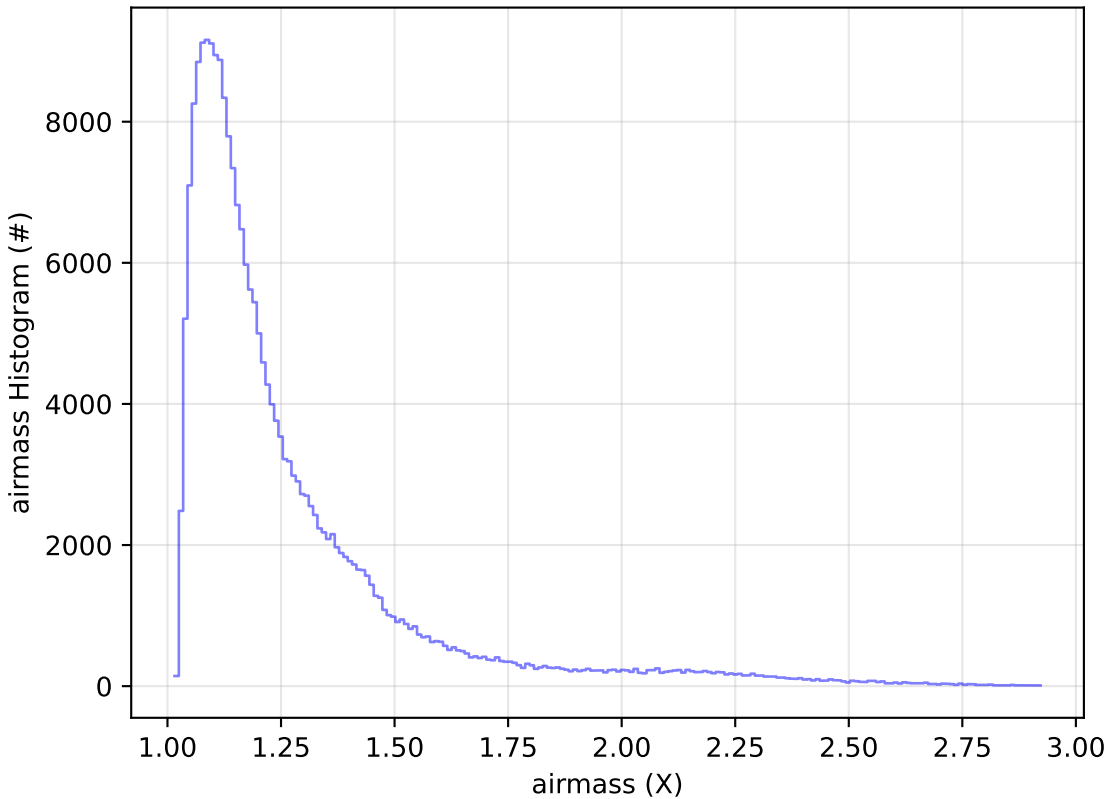
start_date_do-360v3.4_10yrs Yr 1 all bands: airmass Histogram
