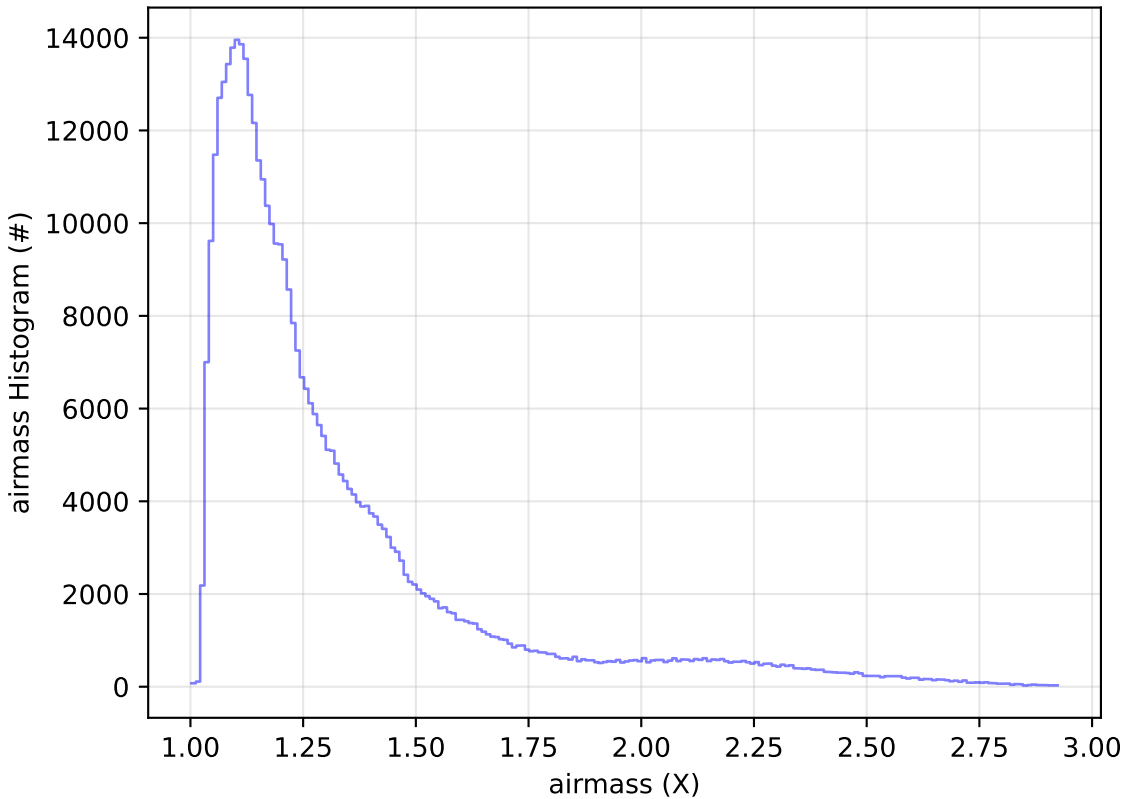
start_date_do-360v3.4_10yrs WFD z band: airmass Histogram
