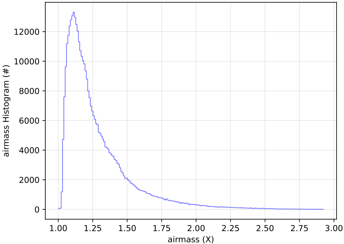
start_date_do-360v3.4_10yrs WFD y band: airmass Histogram
