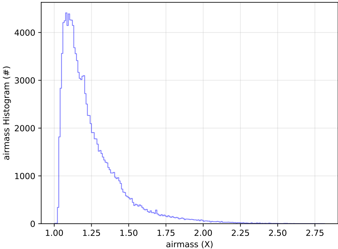
start_date_do-360v3.4_10yrs WFD u band: airmass Histogram
