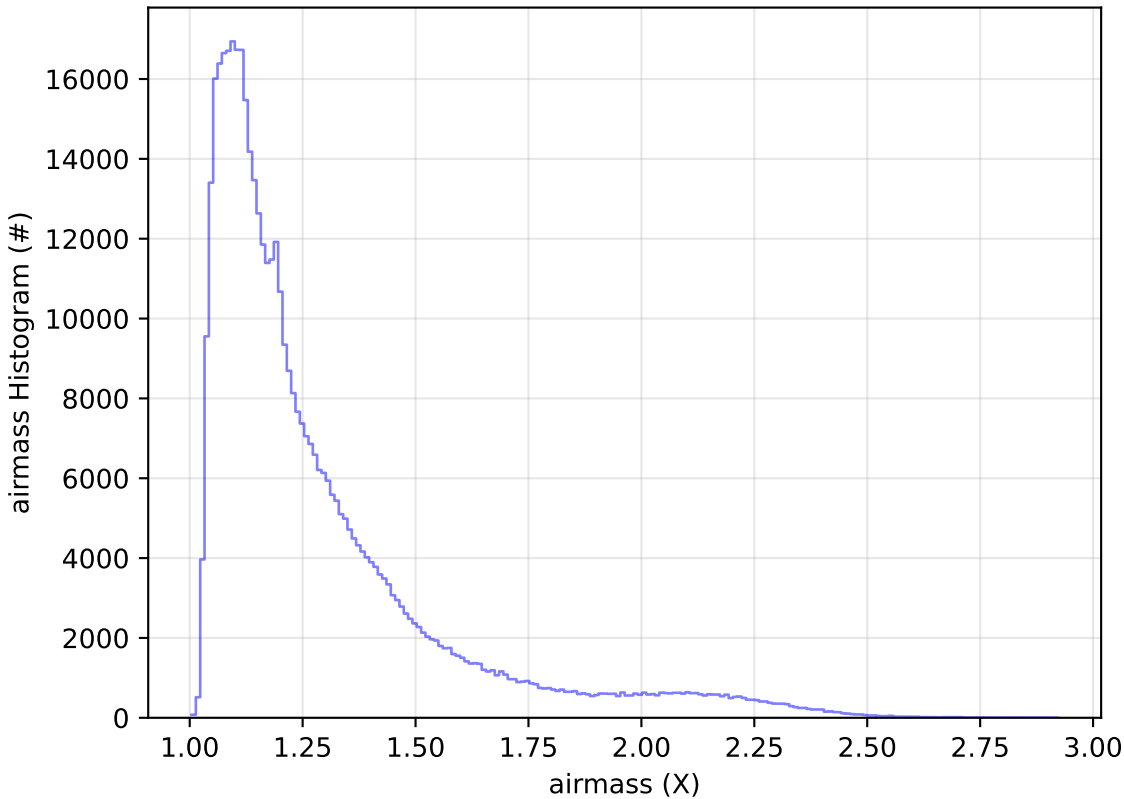
start_date_do-360v3.4_10yrs WFD r band: airmass Histogram
