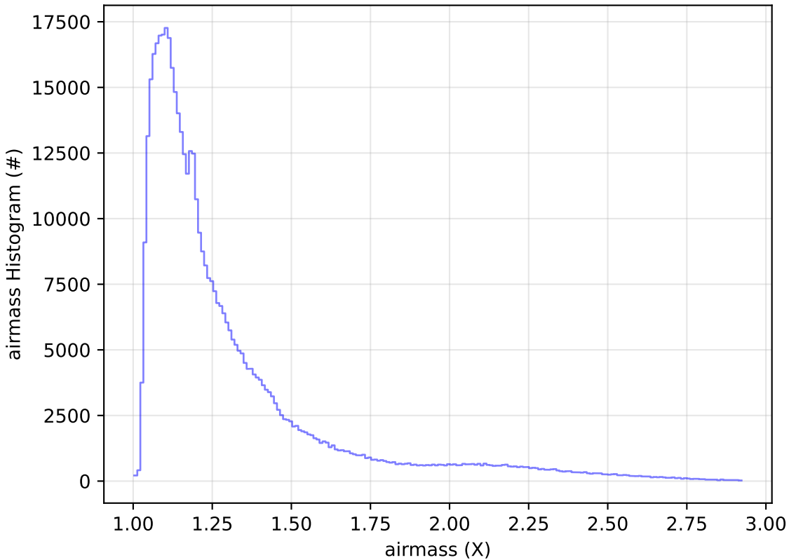
start_date_do-360v3.4_10yrs WFD i band: airmass Histogram
