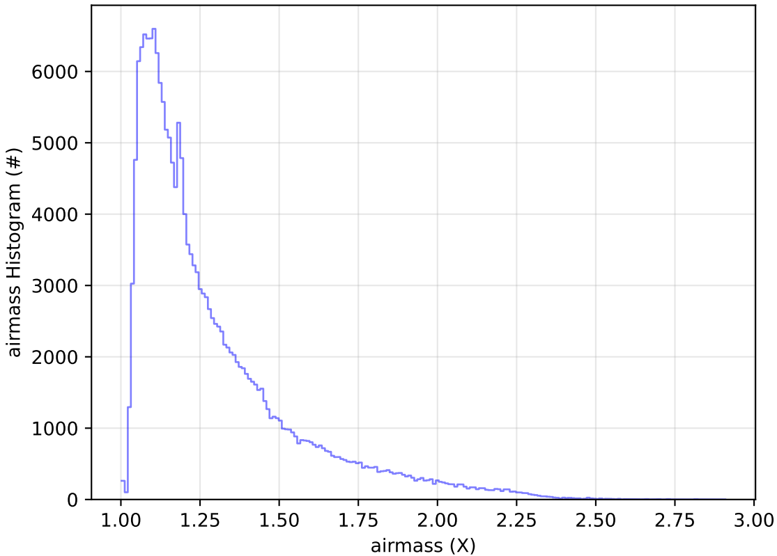
start_date_do-360v3.4_10yrs WFD g band: airmass Histogram
