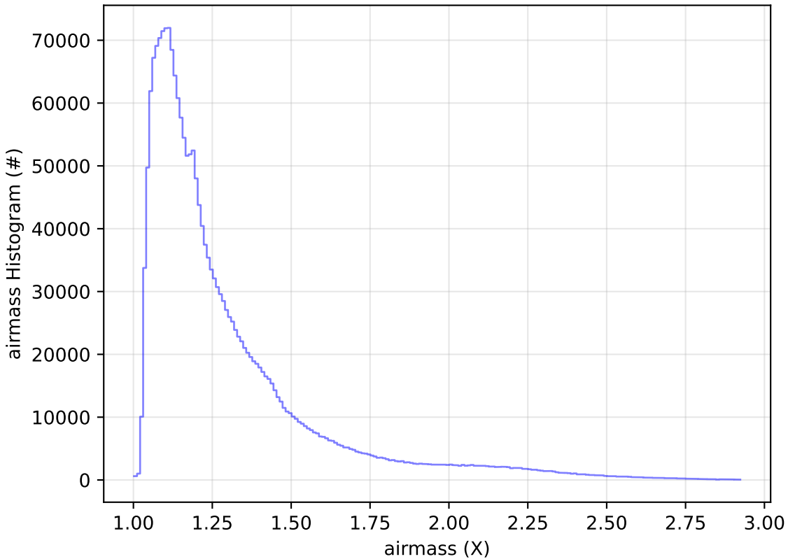
start_date_do-360v3.4_10yrs WFD all bands: airmass Histogram
