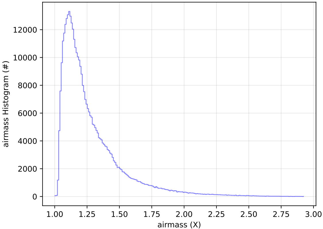
start_date_do-360v3.4_10yrs All sky y band: airmass Histogram
