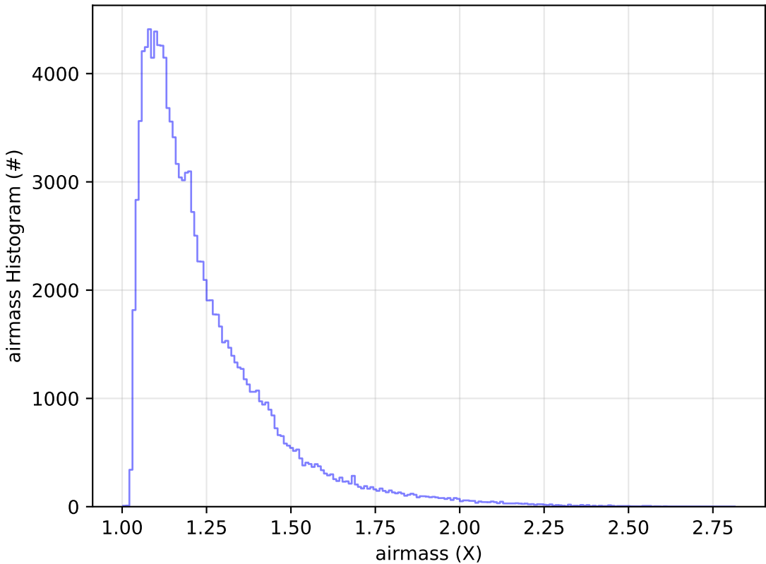
start_date_do-360v3.4_10yrs All sky u band: airmass Histogram
