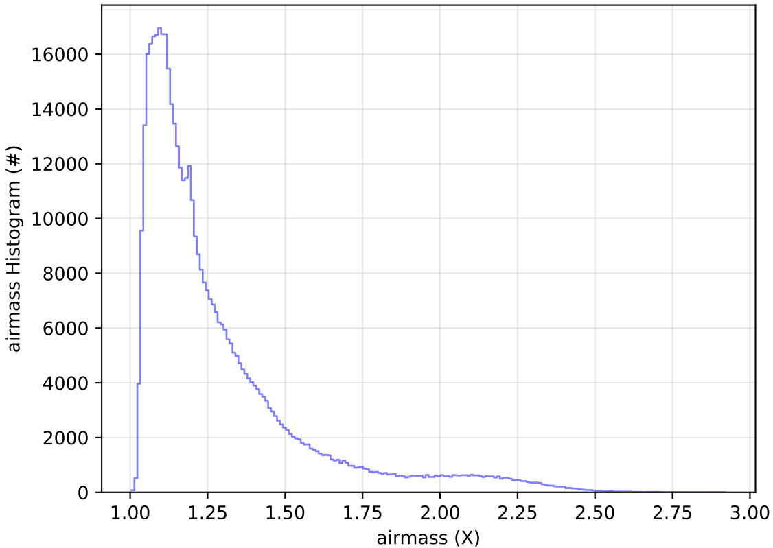
start_date_do-360v3.4_10yrs All sky r band: airmass Histogram
