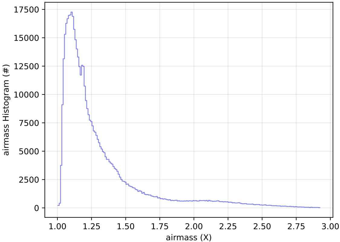
start_date_do-360v3.4_10yrs All sky i band: airmass Histogram
