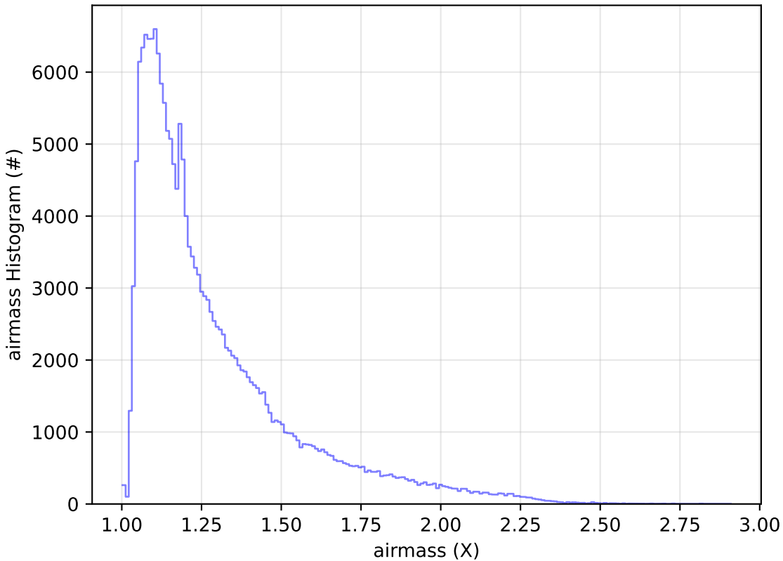
start_date_do-360v3.4_10yrs All sky g band: airmass Histogram
