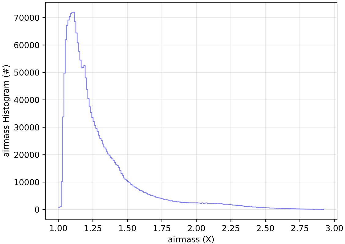
start_date_do-360v3.4_10yrs All sky all bands: airmass Histogram
