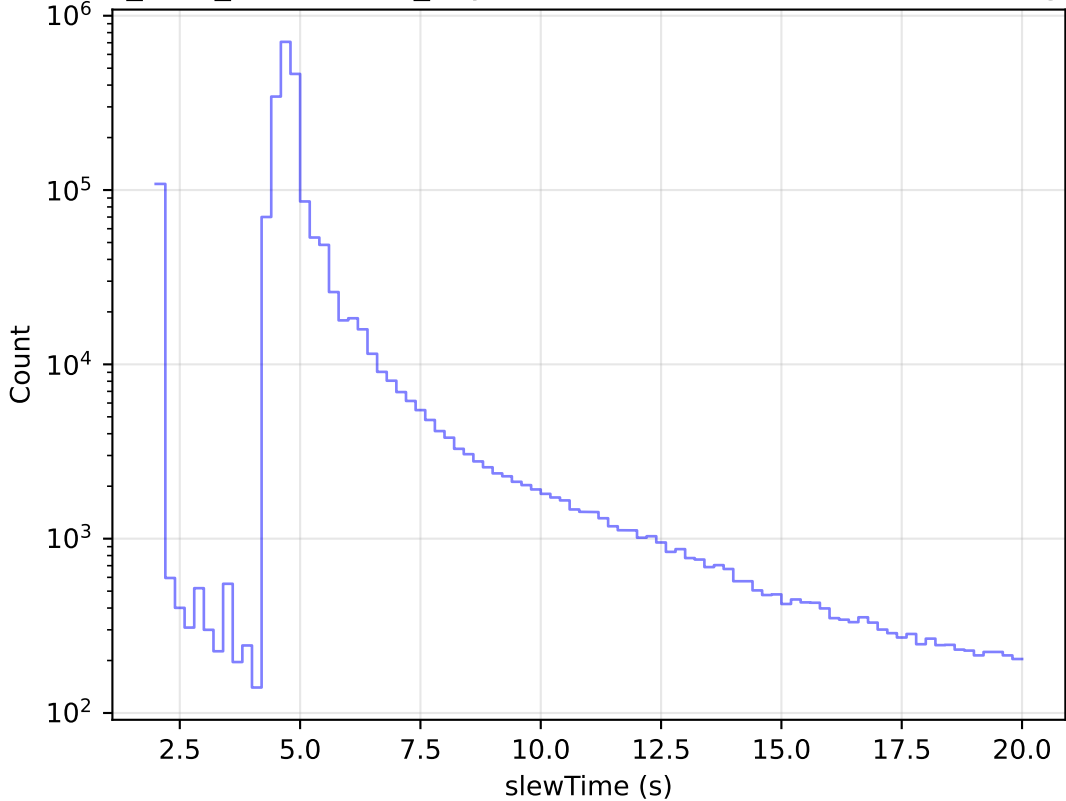
start_date_do-360v3.4_10yrs All visits: Zoom Slew Time Histogram
