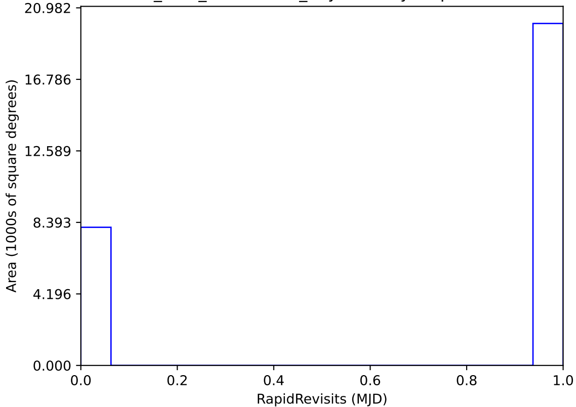
start_date_do-360v3.4_10yrs All sky: RapidRevisits
