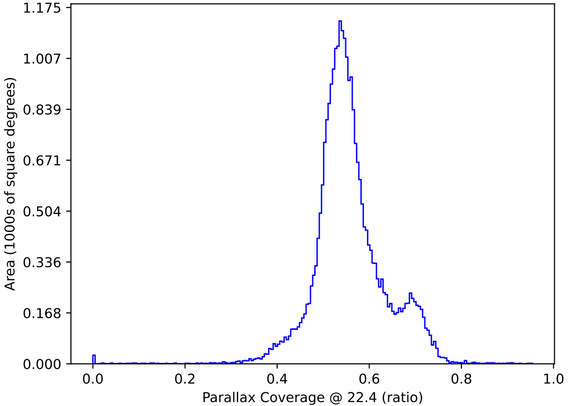
start_date_do-360v3.4_10yrs All sky: Parallax Coverage @ 22.4
