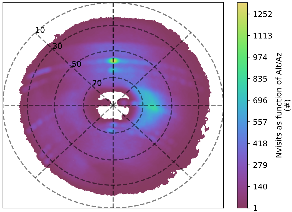
start_date_do-360v3.4_10yrs g band: Nvisits as function of Alt/Az
