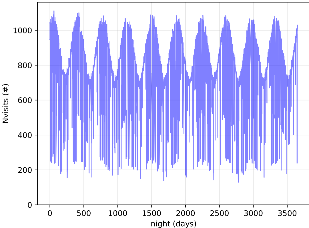
start_date_do-360v3.4_10yrs All visits: Nvisits
