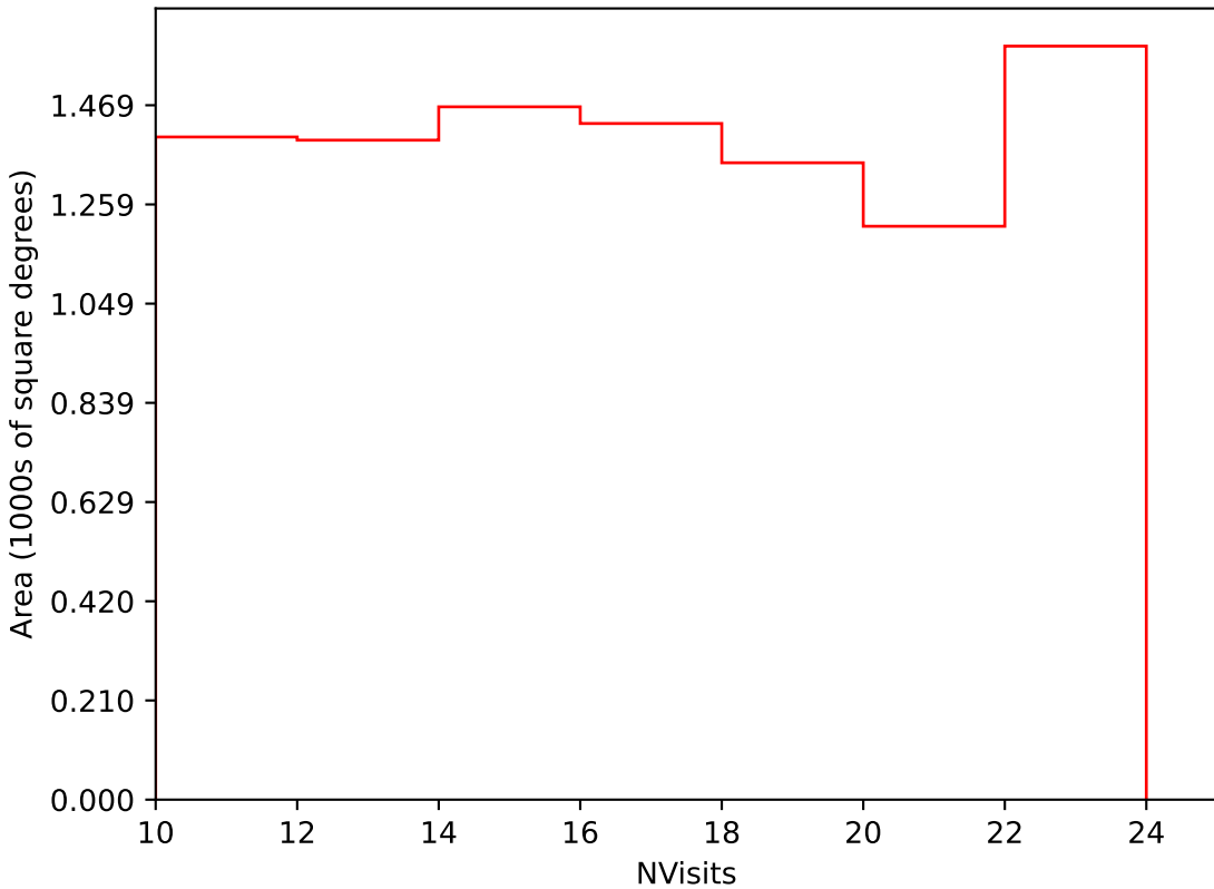
start_date_do-360v3.4_10yrs Yr 3-4 i band: NVisits
