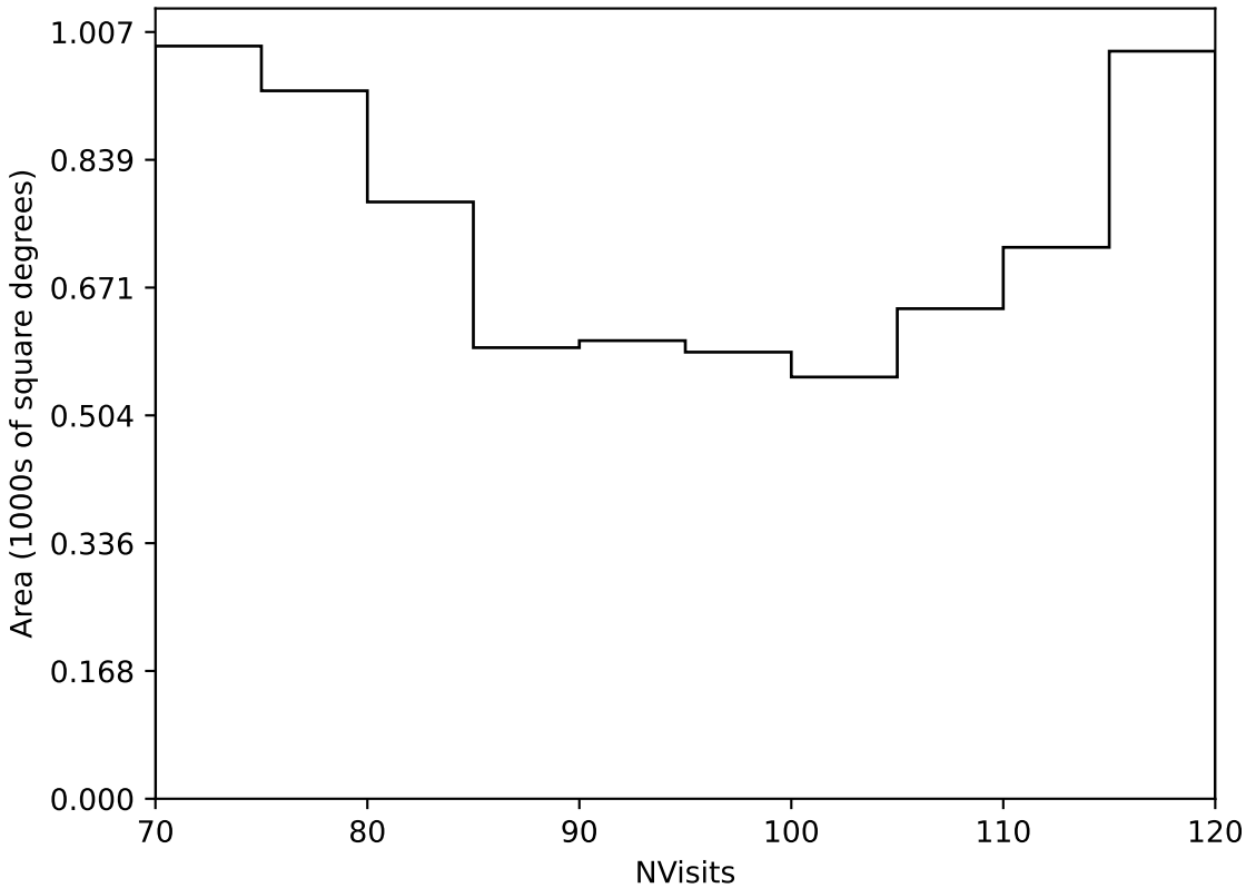
start_date_do-360v3.4_10yrs Yr 3-4 all bands: NVisits
