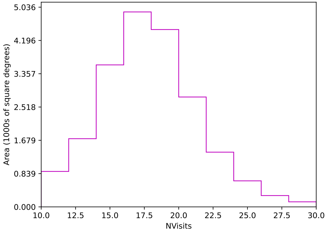
start_date_do-360v3.4_10yrs Yr 1 z band: NVisits
