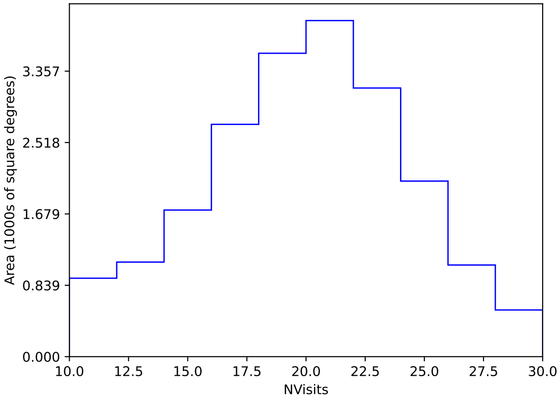
start_date_do-360v3.4_10yrs Yr 1 y band: NVisits
