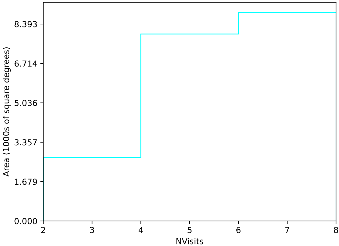
start_date_do-360v3.4_10yrs Yr 1 u band: NVisits
