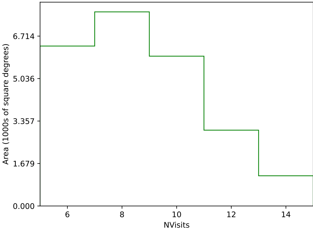
start_date_do-360v3.4_10yrs Yr 1 g band: NVisits
