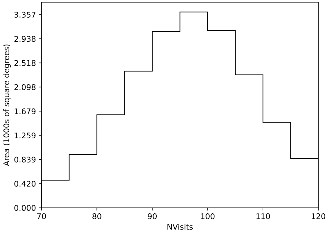
start_date_do-360v3.4_10yrs Yr 1 all bands: NVisits
