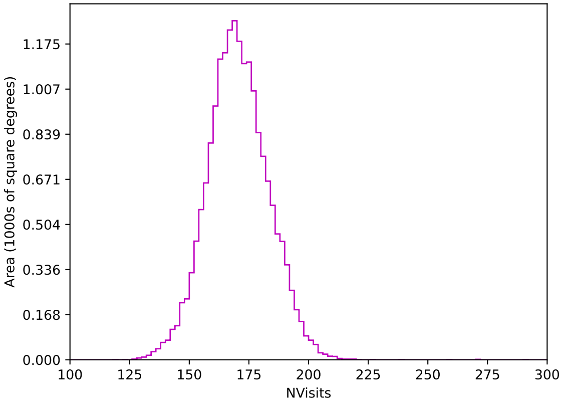
start_date_do-360v3.4_10yrs WFD z band: NVisits
