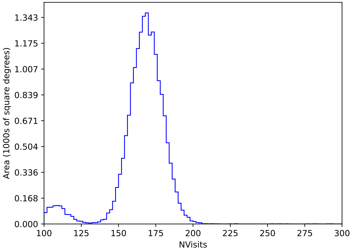
start_date_do-360v3.4_10yrs WFD y band: NVisits
