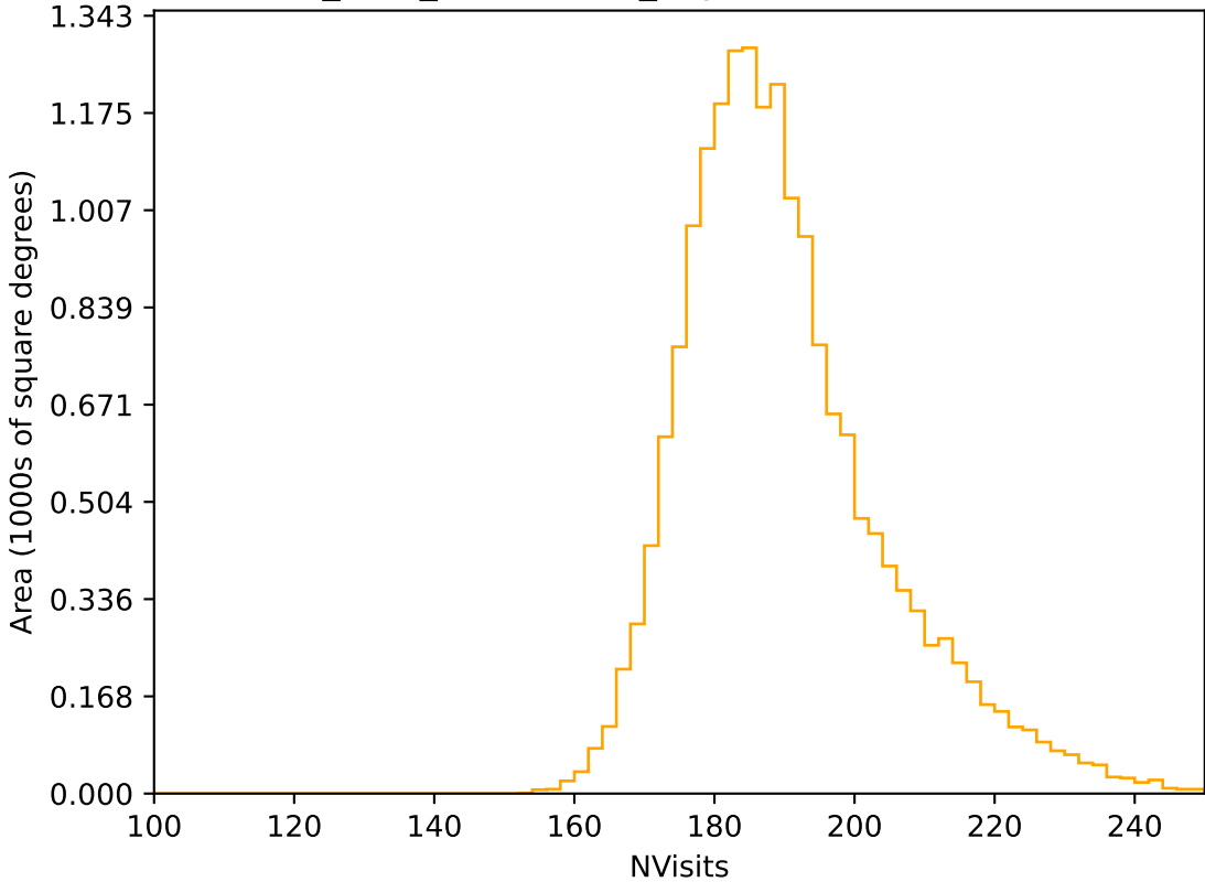
start_date_do-360v3.4_10yrs WFD r band: NVisits
