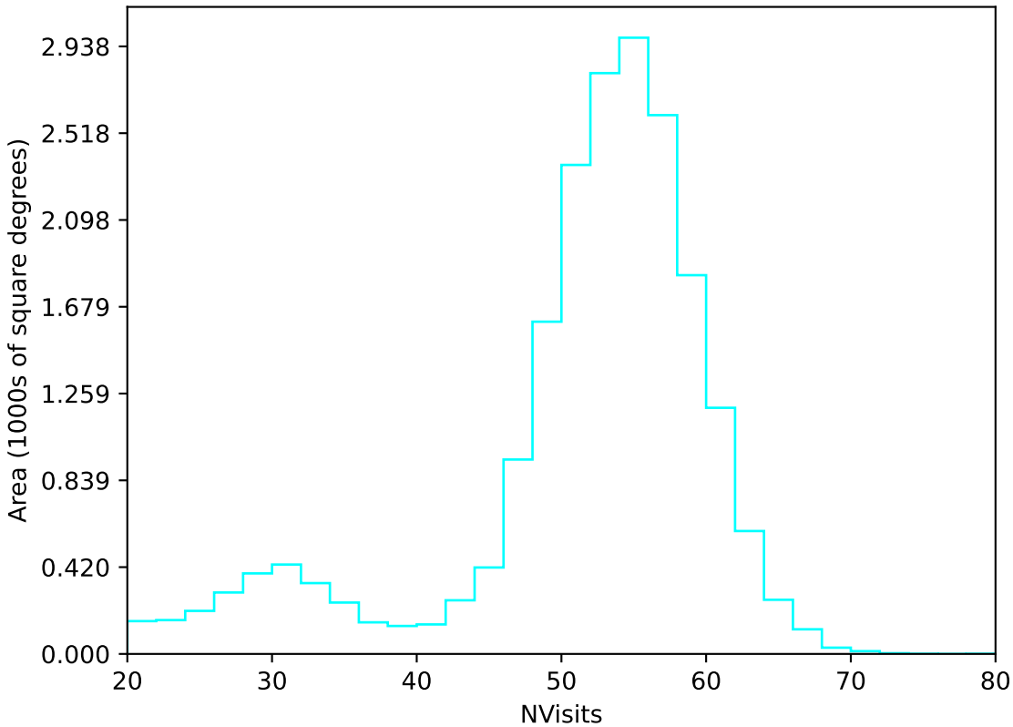
start_date_do-360v3.4_10yrs All sky u band: NVisits
