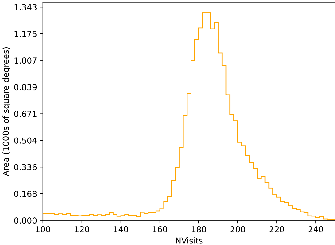
start_date_do-360v3.4_10yrs All sky r band: NVisits
