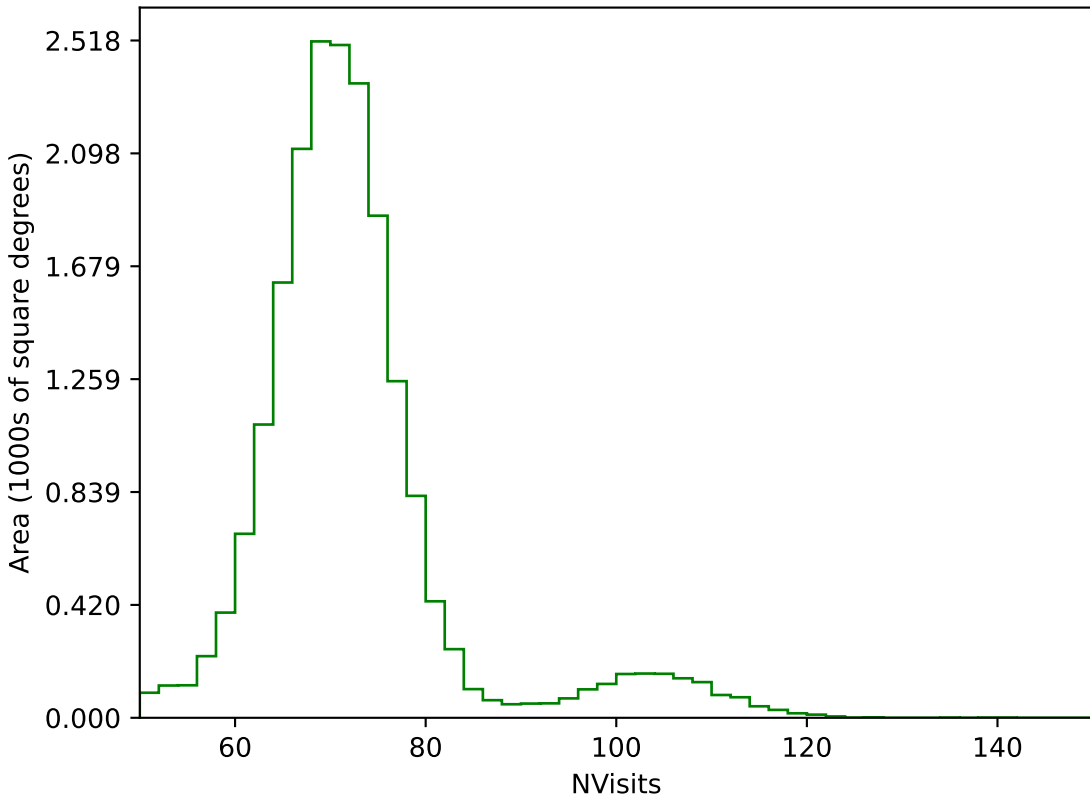
start_date_do-360v3.4_10yrs All sky g band: NVisits
