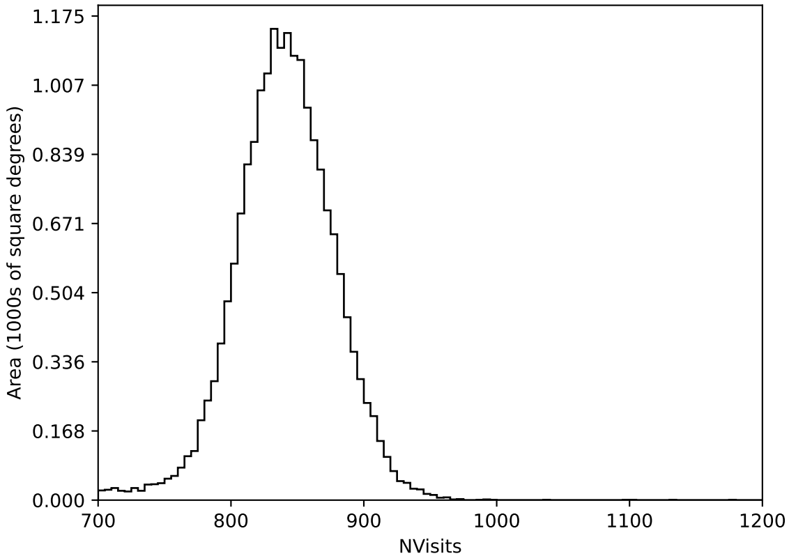
start_date_do-360v3.4_10yrs All sky all bands: NVisits
