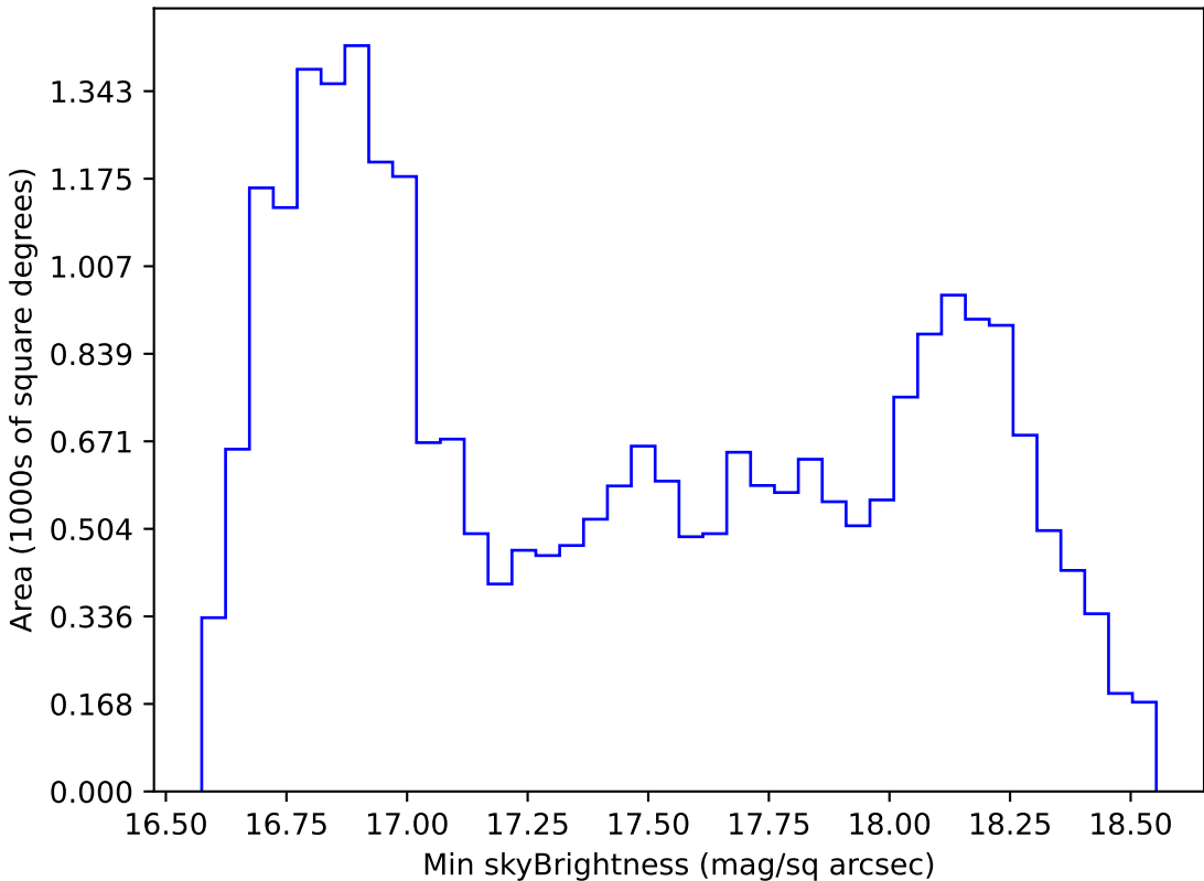
start_date_do-360v3.4_10yrs All sky z band: Min skyBrightness
