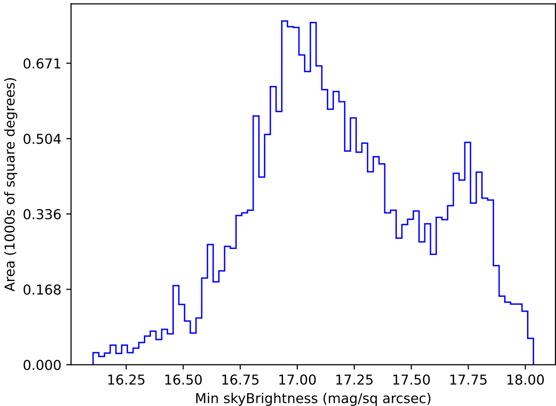
start_date_do-360v3.4_10yrs All sky y band: Min skyBrightness
