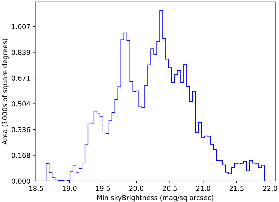
start_date_do-360v3.4_10yrs All sky g band: Min skyBrightness
