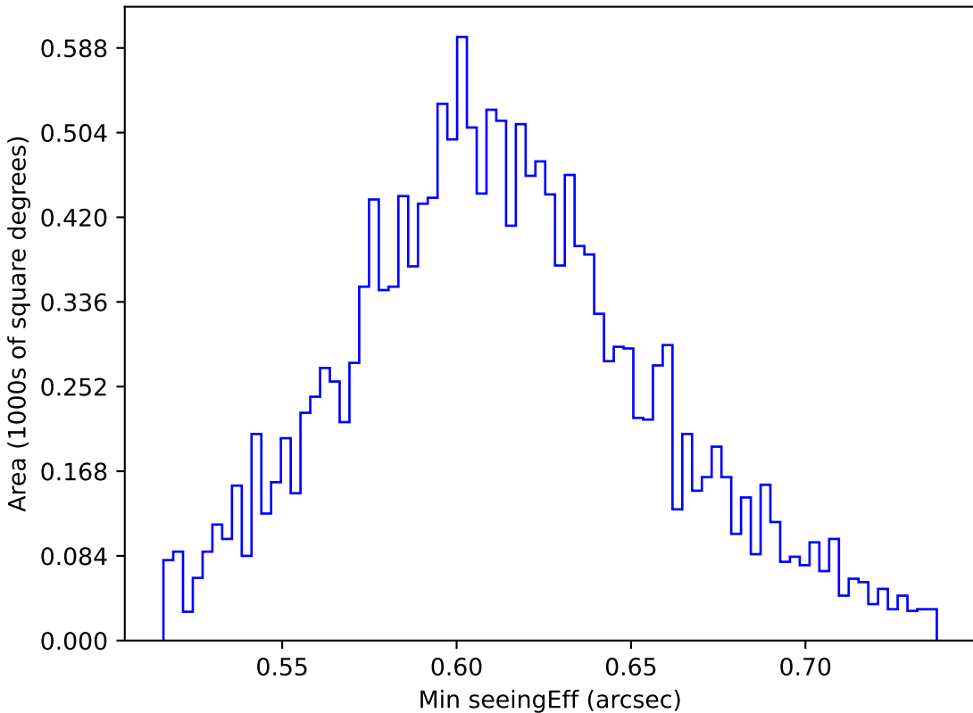
start_date_do-360v3.4_10yrs WFD z band: Min seeingEff
