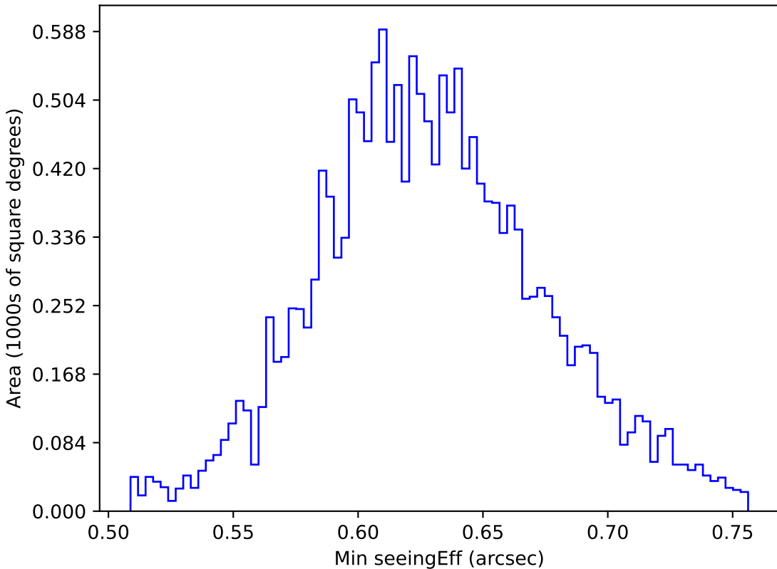
start_date_do-360v3.4_10yrs WFD y band: Min seeingEff
