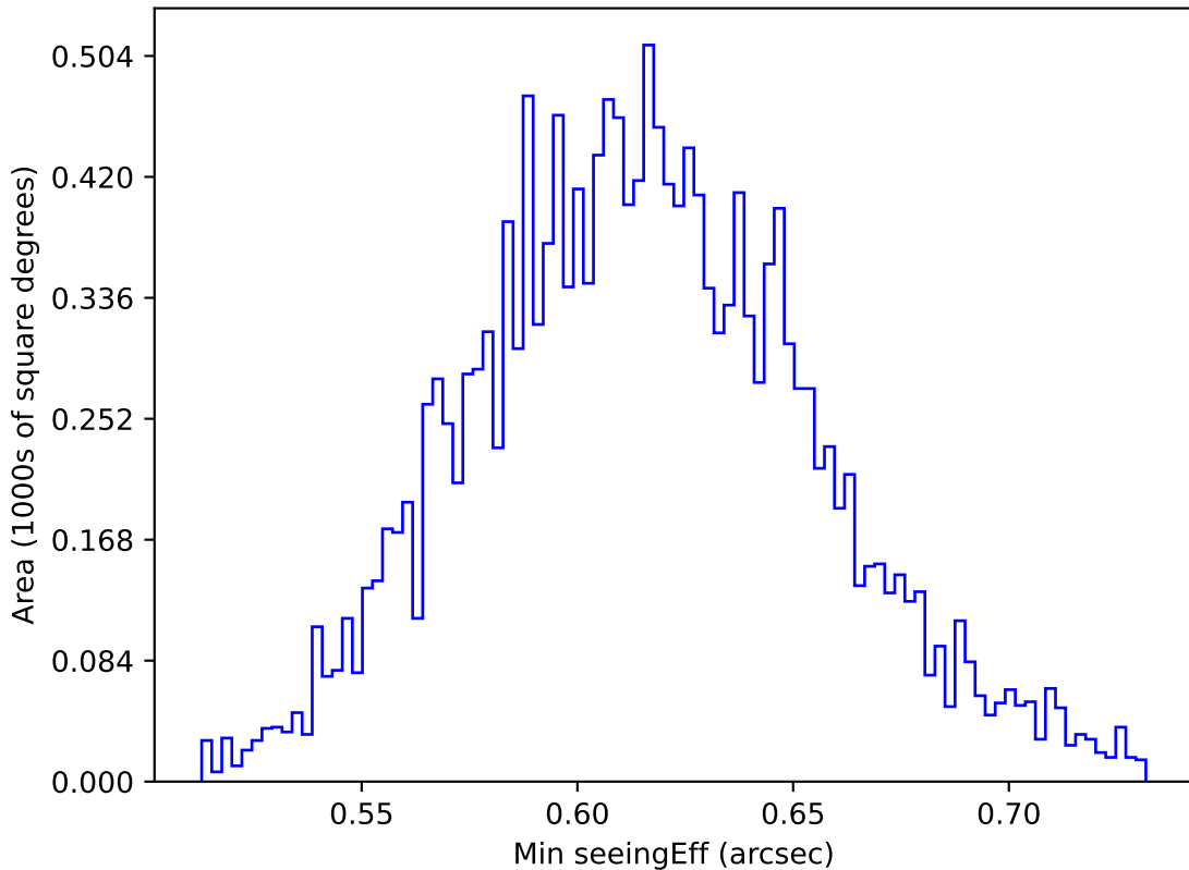
start_date_do-360v3.4_10yrs WFD r band: Min seeingEff
