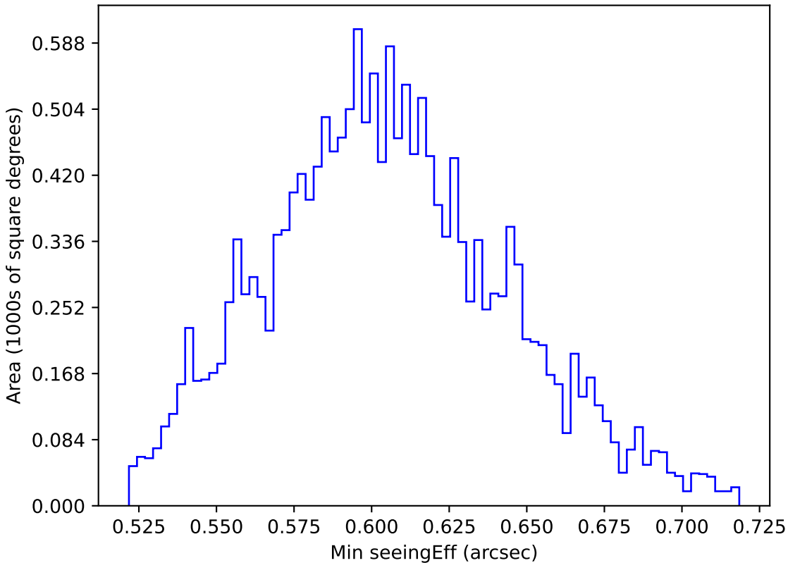
start_date_do-360v3.4_10yrs WFD i band: Min seeingEff
