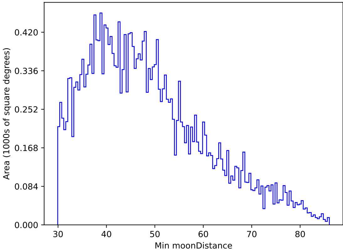
start_date_do-360v3.4_10yrs All sky g band: Min moonDistance
