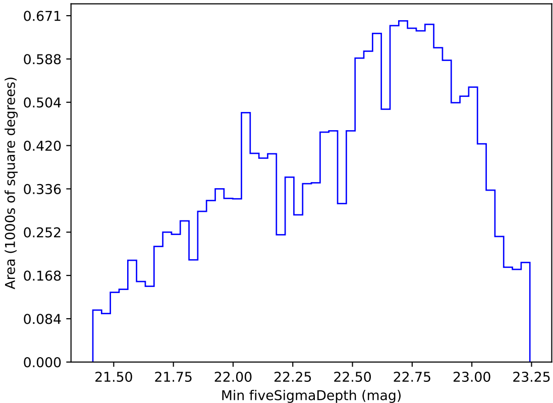
start_date_do-360v3.4_10yrs WFD r band: Min fiveSigmaDepth
