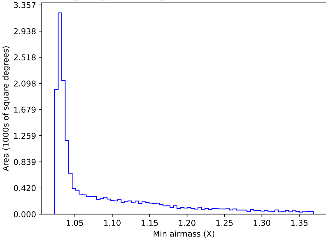
start_date_do-360v3.4_10yrs WFD y band: Min airmass
