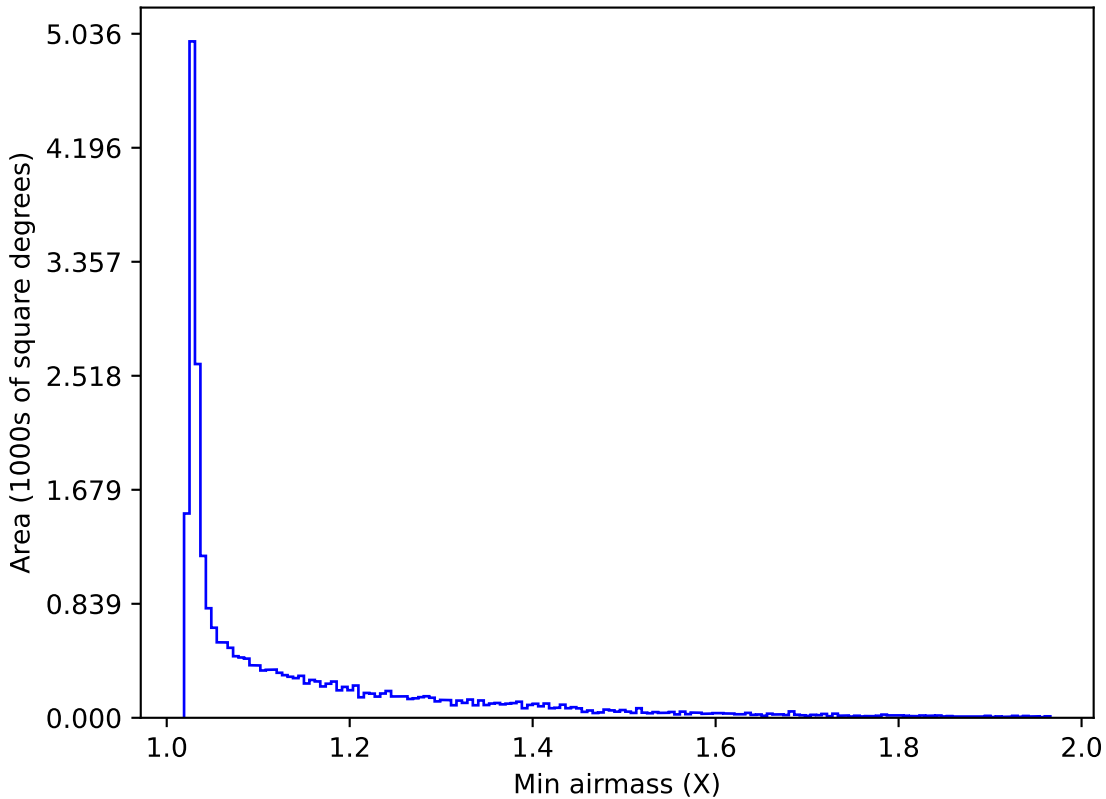
start_date_do-360v3.4_10yrs All sky z band: Min airmass
