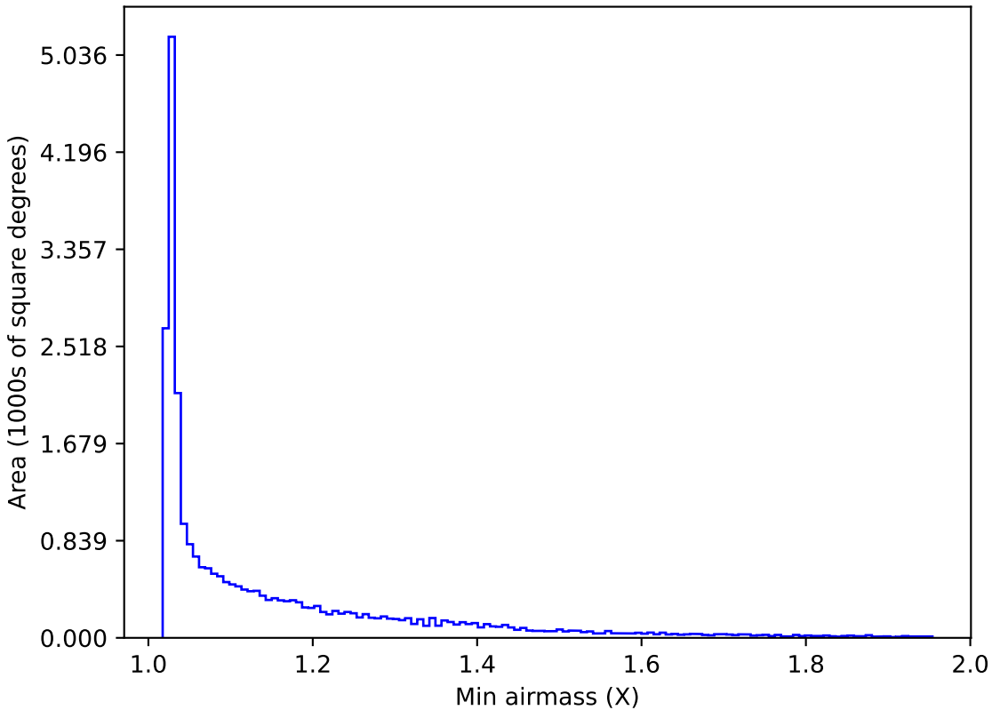
start_date_do-360v3.4_10yrs All sky r band: Min airmass
