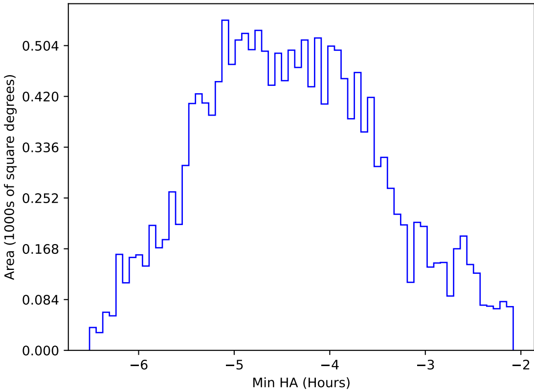
start_date_do-360v3.4_10yrs WFD z band: Min HA
