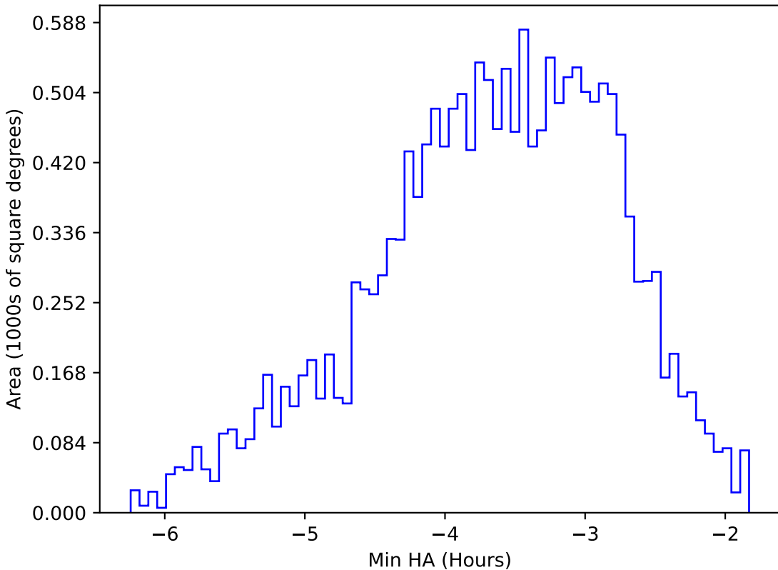
start_date_do-360v3.4_10yrs WFD y band: Min HA
