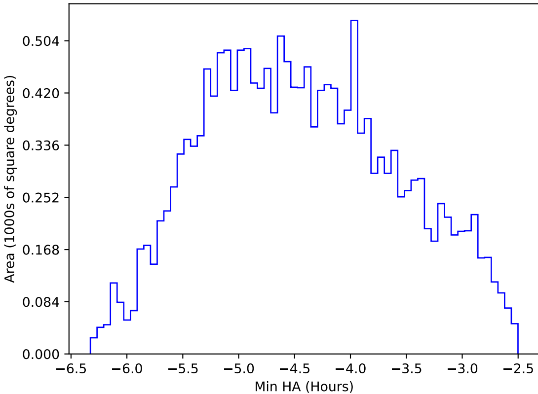
start_date_do-360v3.4_10yrs WFD r band: Min HA
