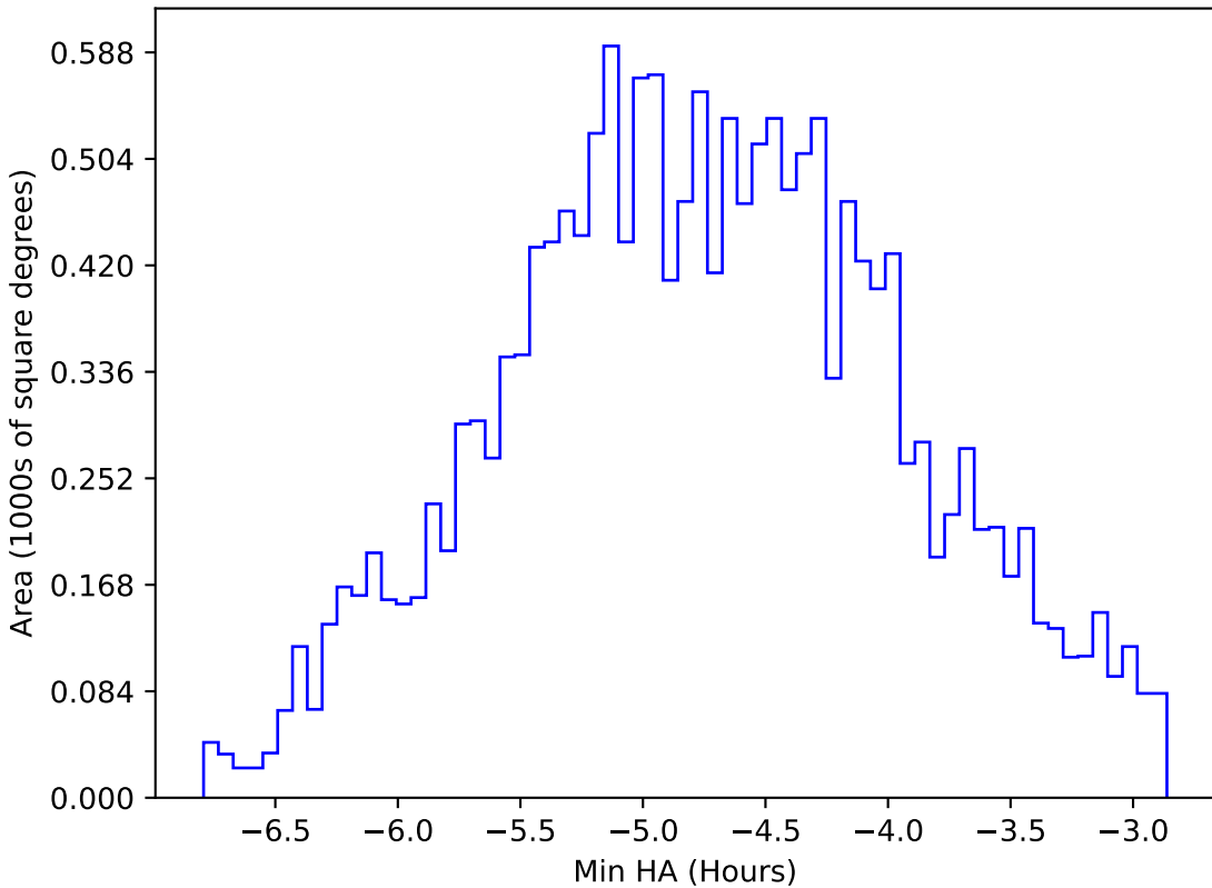
start_date_do-360v3.4_10yrs WFD all bands: Min HA
