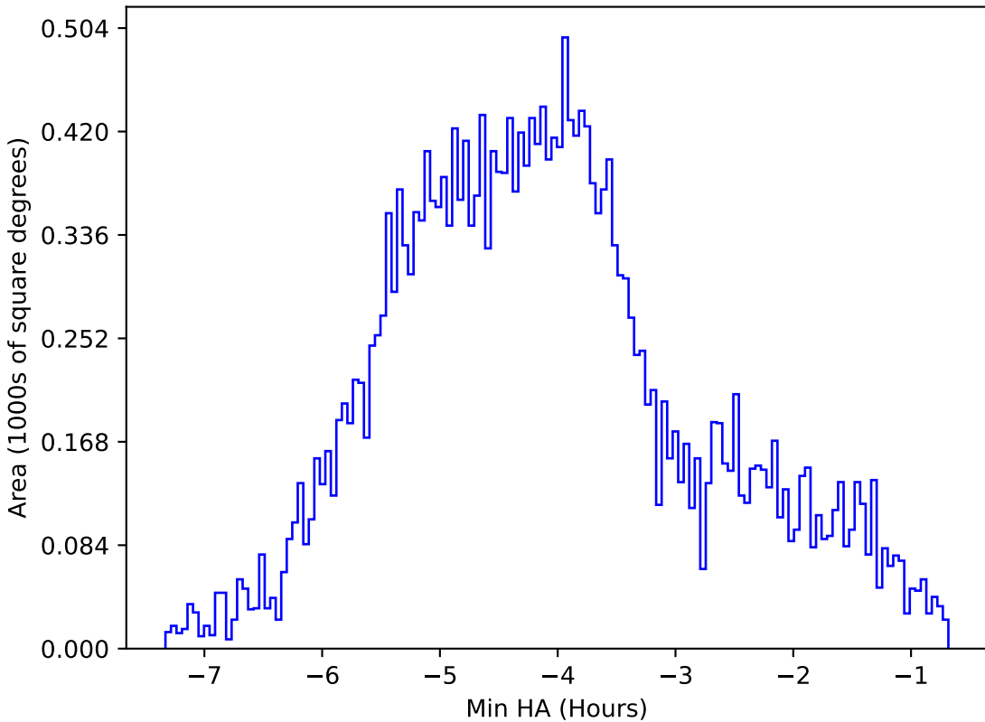
start_date_do-360v3.4_10yrs All sky z band: Min HA
